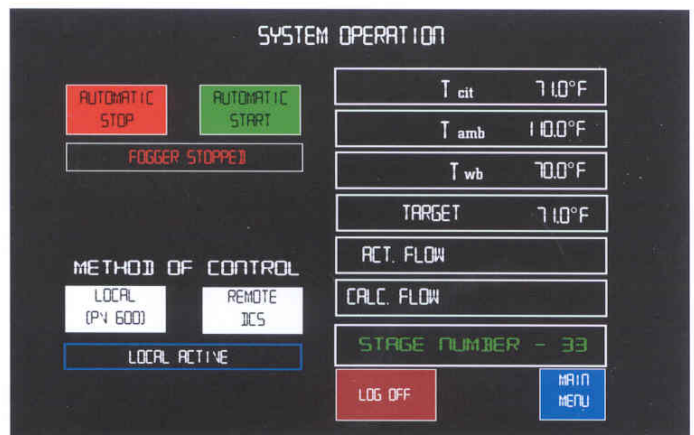
Typical Operator Screen Using Panel View
