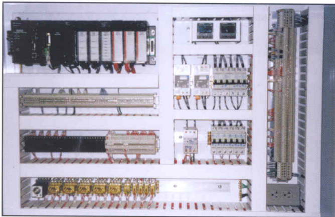
PLC Panel
