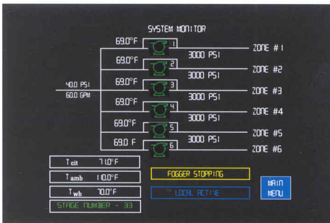
Typical Operator Screen Using Panel View
